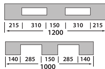
Forklift Entry Dimensions
